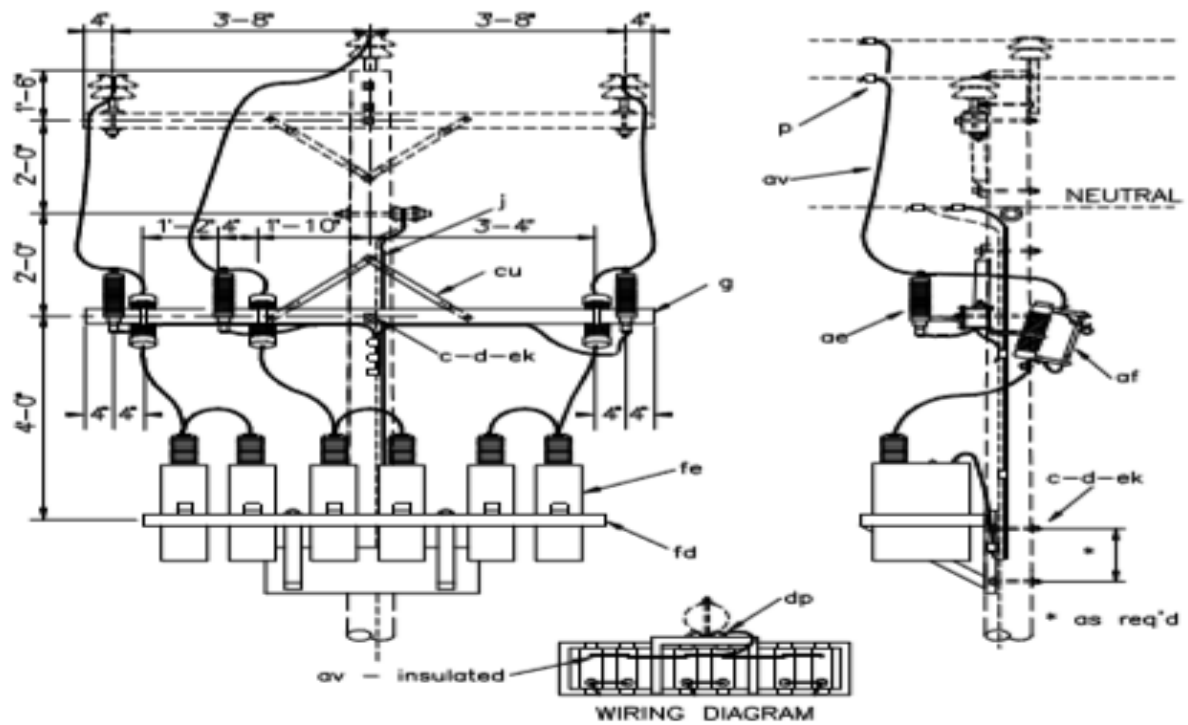
WIRING DIAGRAM
